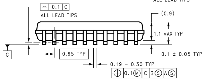
20-Lead Molded TSSOP, Exposed Pad, 6.5x4.4x0.9mm Order Number HWD4863MTE HWD Package Number MXA20A
